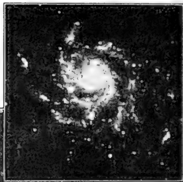
Above: Spiral nebula Messier 101, Ursa Majoris, photographed with the two-foot reflector of the Yerkes Observatory. Time of exposure, three hours
